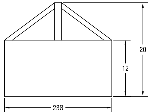
Scum baffle
